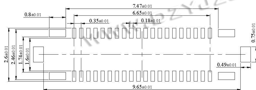
RECOMMENDED METAL DIMENSIONS (THICKNESS: 0.08 mm)
